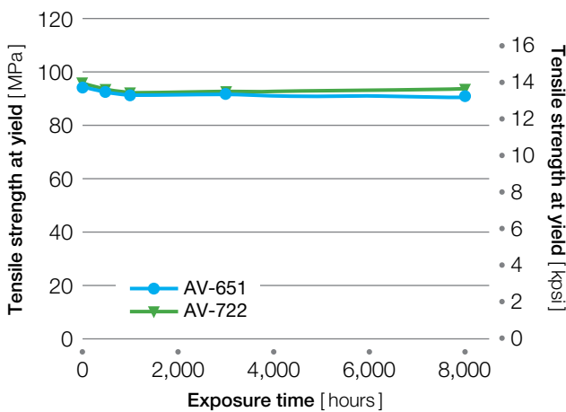
Figure 7.14 Tensile strength at yield
