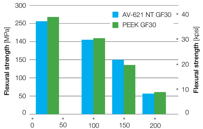
Figure 3.26 Flexural strength of AvaSpire® AV-621 GF30 BG20 and 30 % GF PEEK
