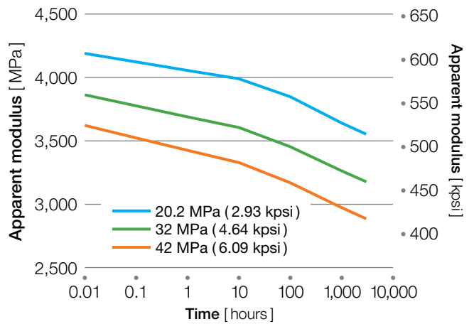
Figure 4.6 AV-722 BG20 at 23 °C (73 °F)
