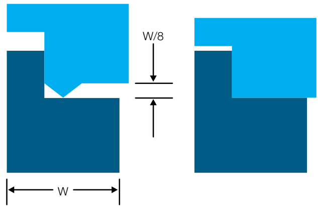
Figure 10.4 Step joint
