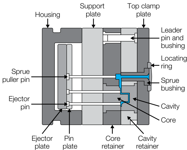
Figure 9.17 Two plate tool
