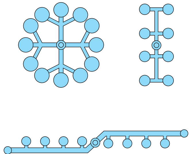
Figure 9.19 Unbalanced
