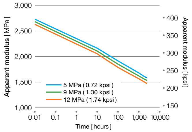
Figure 4.10 AV-722 BG20 at 120 °C (248 °F)
