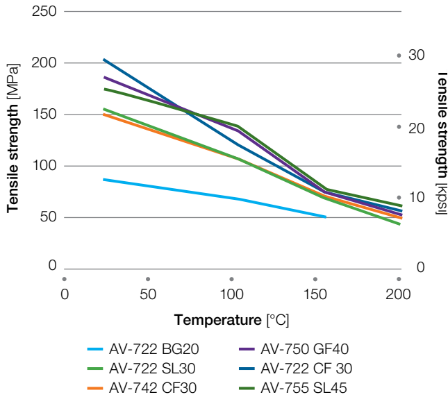
Figure 3.8 Tensile strength vs. temperature AvaSpire® AV-700 Series
