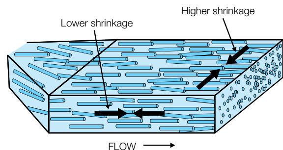
Figure 9.22 Shrinkage varies with flow direction
