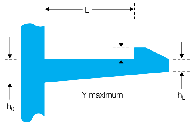
Figure 8.13 Snap fit design using tapered beam
