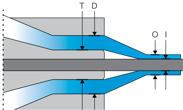
Figure 9.37 Sleeve die draw down ratio
