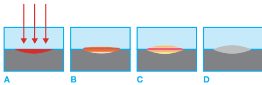
Figure 10.7 Laser welding process
