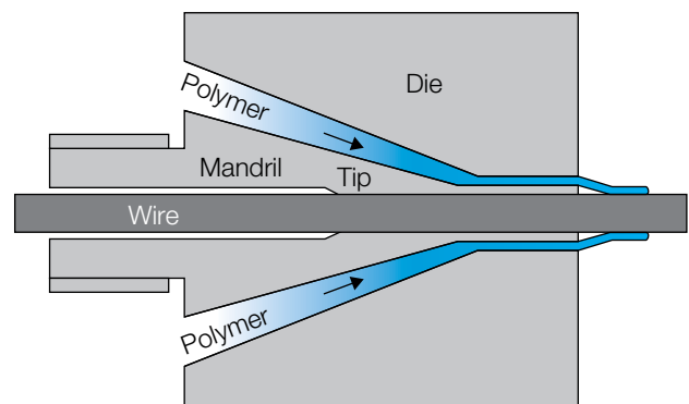
Figure 9.36 Schematic of sleeve die
