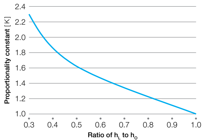
Figure 8.14 Proportionality constant ( K ) for tapered beam
