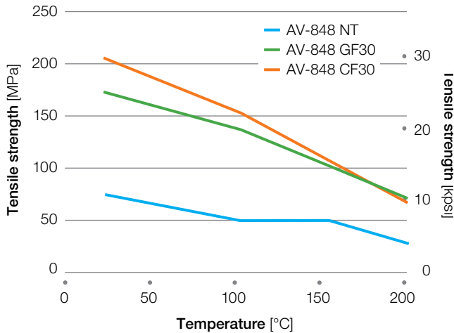
Figure 3.9 Tensile strength vs. temperature AvaSpire® AV-800 series
