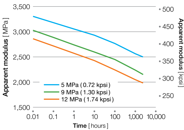
Figure 4.9 AV-621 NT at 120 °C (248 °F)
