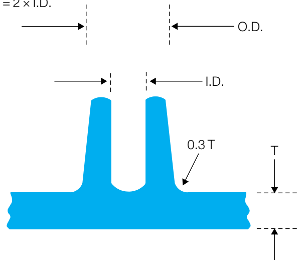
Figure 8.18 Boss design – general guidelines
