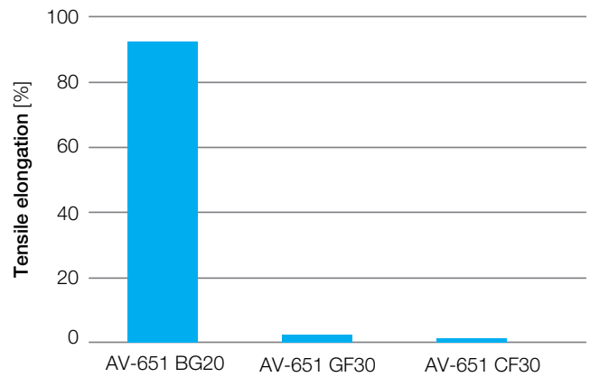
Figure 3.6 Tensile elongation and fiber reinforcement
