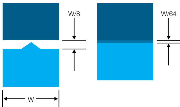
Figure 10.3 Butt joint
