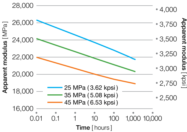
Figure 4.13 AV-848 CF30 at 120 °C (248 °F)
