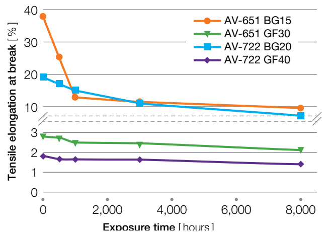
Figure 7.17 Tensile elongation at break
