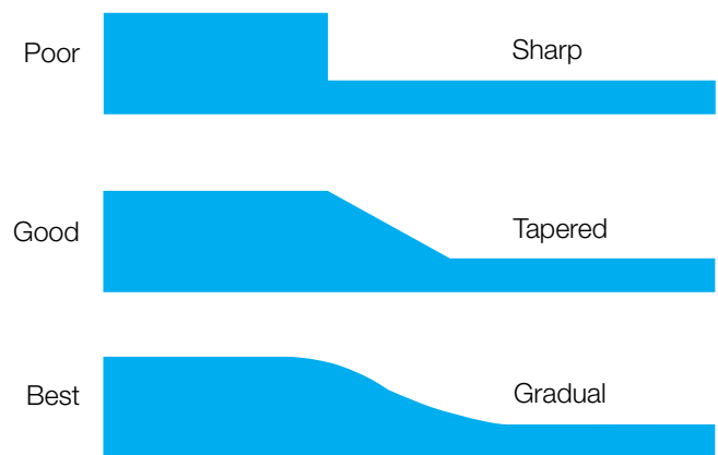
Figure 8.15 Wall thickness transition
