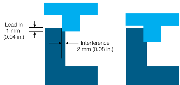
Figure 10.6 Shear joint
