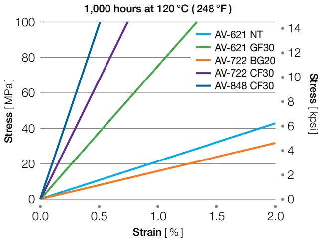
Figure 4.2 Isochronous curves at 120 °C (248 °F)
