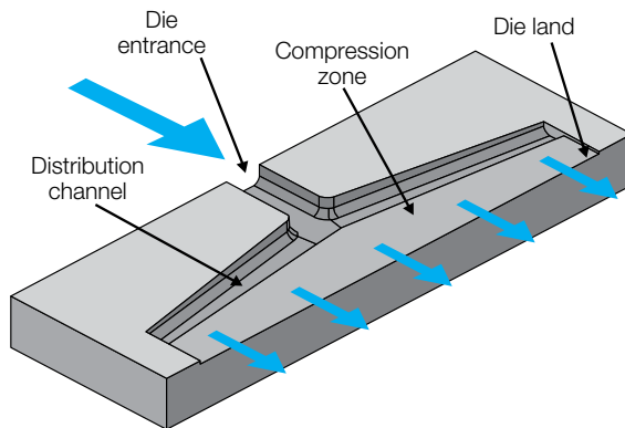
Figure 9.29 Coat hanger film die conceptual lower die plate
