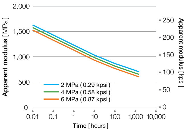
Figure 4.14 AV-621 NT at 160 °C (320 °F)
