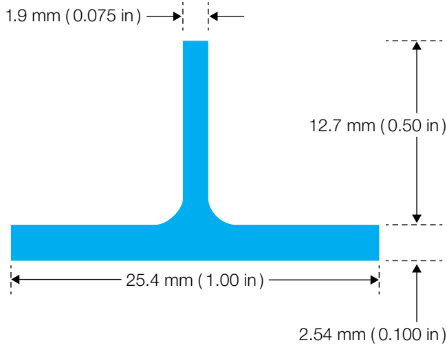
Figure 8.5 Rib design example
