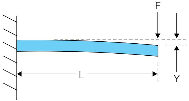
Figure 8.12 Cantilever beam with concentrated load at free end
