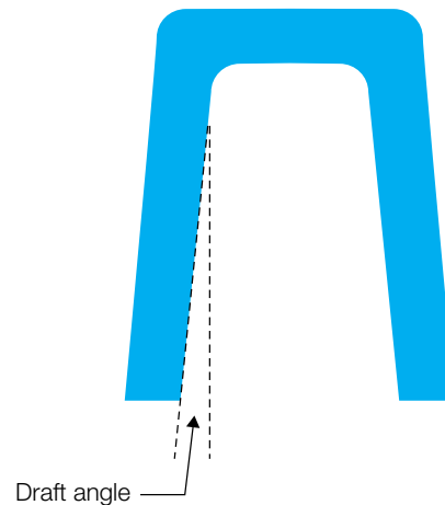
Figure 8.16 Draft – designing for mold release
