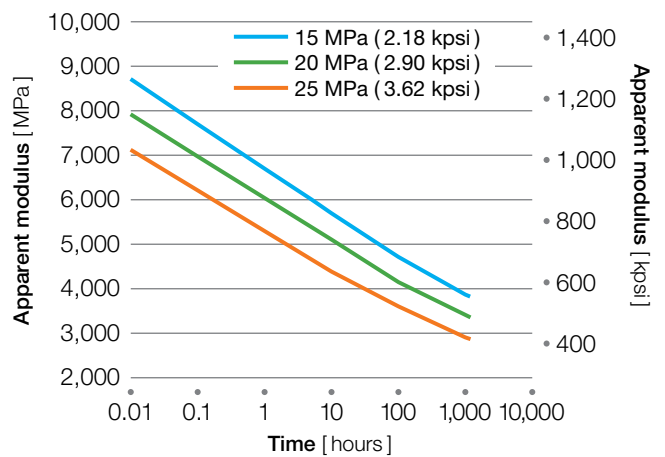
Figure 4.18 AV-848 CF30 at 200 °C (392 °F)
