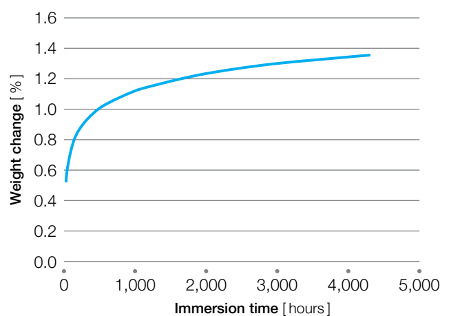
Figure 7.20 Water absorption of AvaSpire® 848 NT
