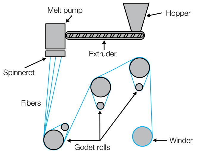
Figure 9.33 Fiber spinning process
