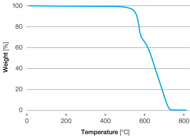
Figure 5.10 TGA AV-630 NT in Air
