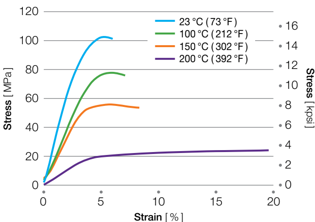
Figure 3.29 Stress-strain curves for AvaSpire® AV-621 NT
