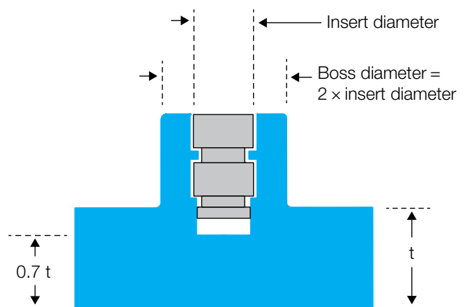
Figure 8.10 Boss design for ultrasonic inserts
