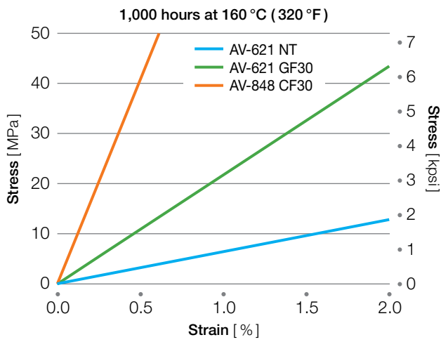
Figure 4.3 Isochronous curves at 160 °C (320 °F)
