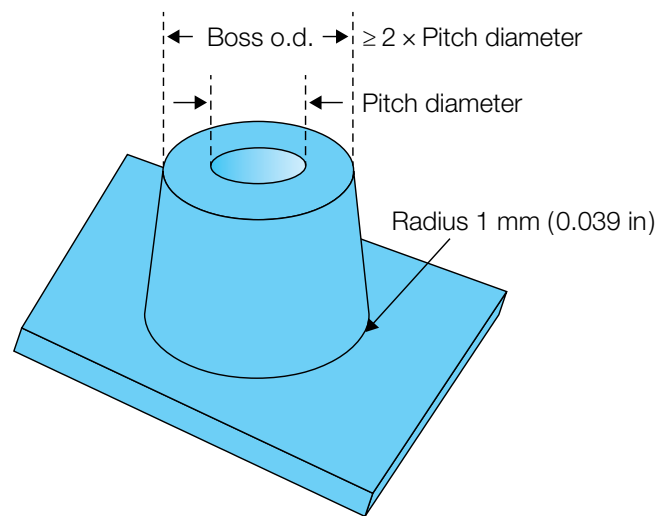
Figure 8.8 Boss design for self-tapping screws
