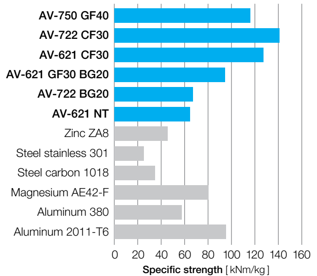
Figure 8.1 Specific strength comparison
