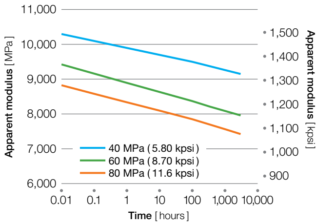
Figure 4.7 AV-621 GF30 at 23 °C (73 °F)
