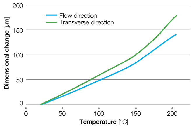
Figure 5.3 CLTE for AvaSpire® AV-621 NT
