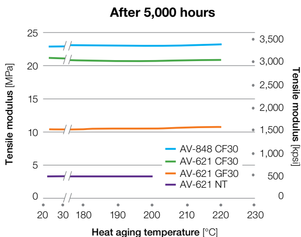
Figure 5.6 Tensile modulus 1
