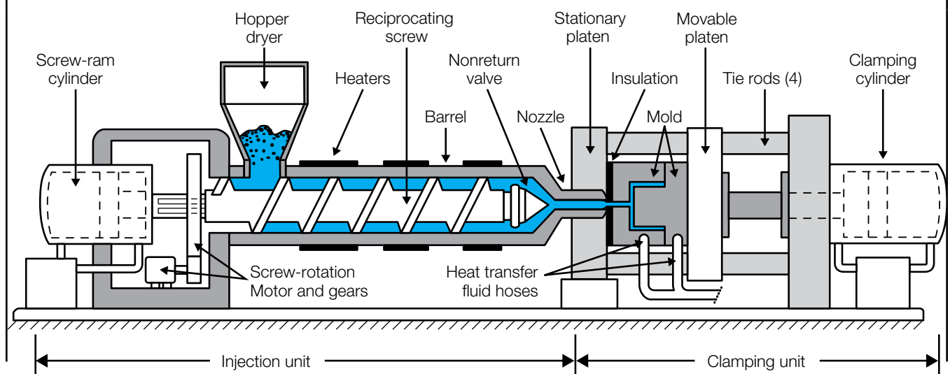
Figure 9.15 Injection molding machine schematic
