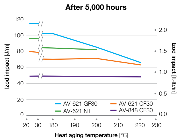
Figure 5.8 Notched Izod impact 1
