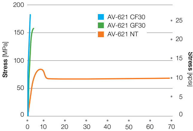
Figure 3.3 Room temperature stress/strain curves for neat and fiber-reinforced grades
