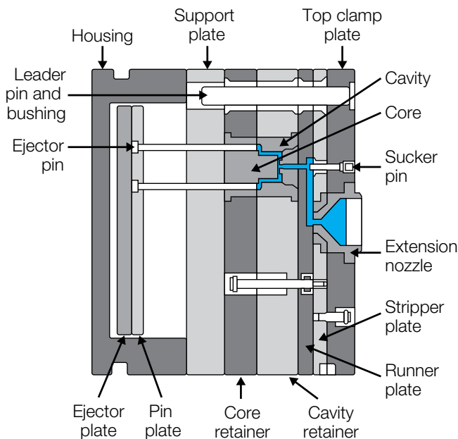
Figure 9.18 Three plate tool
