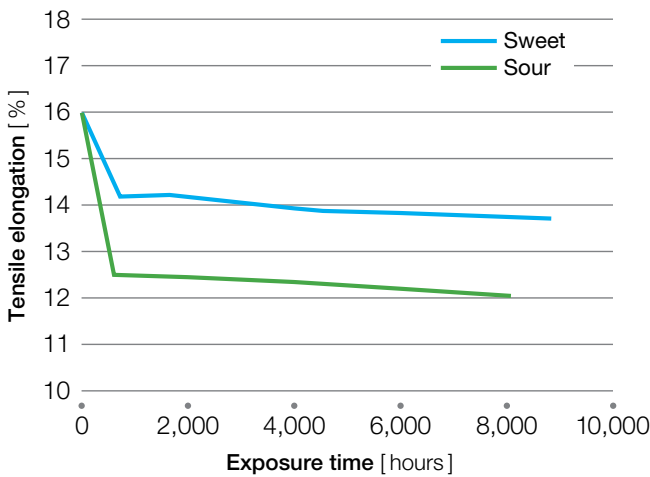
Figure 7.3 Tensile elongation of AV-621 NT exposed at 170 °C (338 °F)
