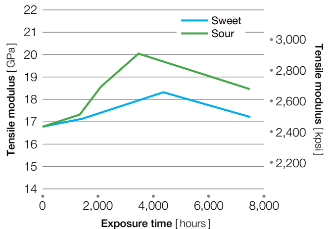
Figure 7.7 Tensile modulus of AV-621 CF30 exposed at 170 °C (338 °F)
