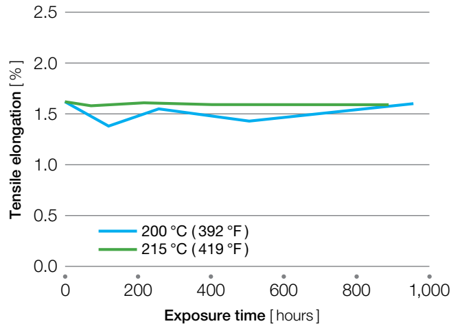
Figure 7.12 Tensile elongation of AV-621 CF30 after high-temperature aging
