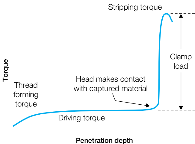
Figure 8.9 Torque developed during screw installation
