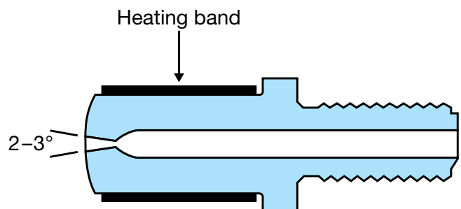
Figure 9.16 Nozzle with reverse taper
