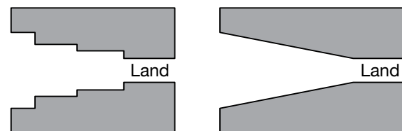
Figure 9.28 Adapter design
