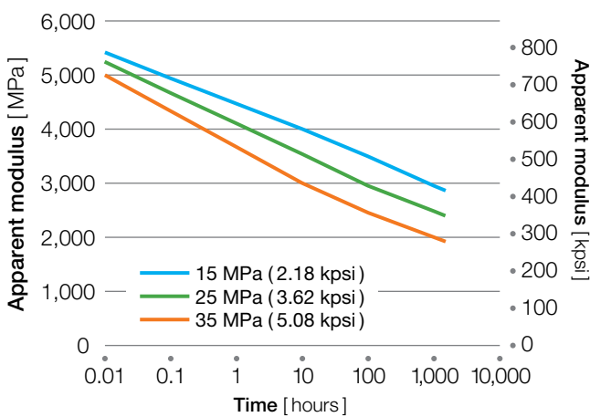
Figure 4.15 AV-621 GF30 at 160 °C (320 °F)
