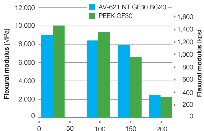
Figure 3.28 Flexural modulus of AvaSpire® AV-621 GF30 BG20 and 30 % GF PEEK
