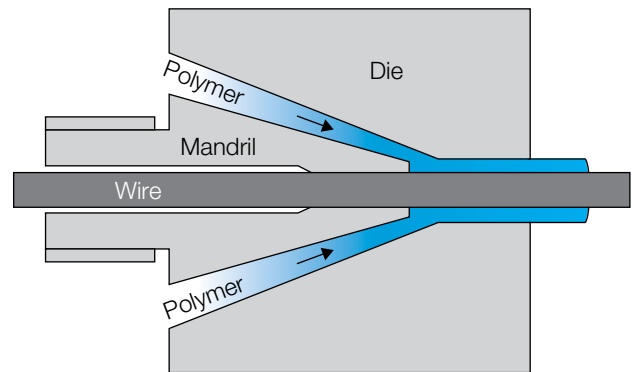
Figure 9.35 Schematic of pressure die
