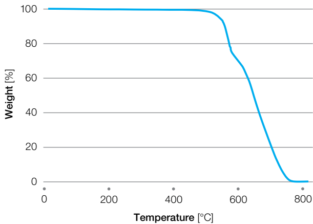
Figure 5.9 TGA AV-621 NT in Air
