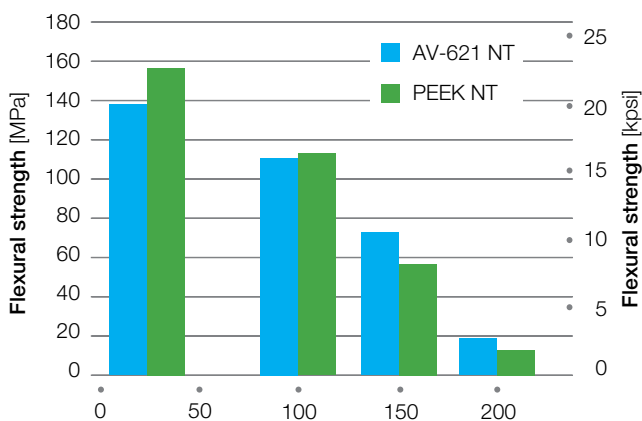
Figure 3.25 Flexural strength of AvaSpire® AV-621 NT and PEEK
