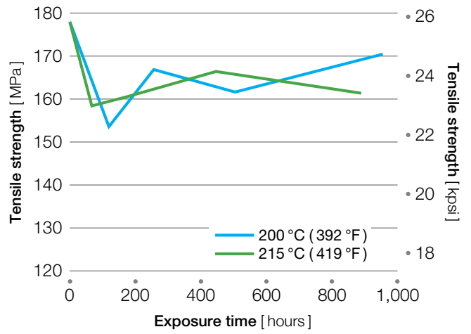
Figure 7.11 Tensile strength of AV-621 CF30 after high-temperature aging
