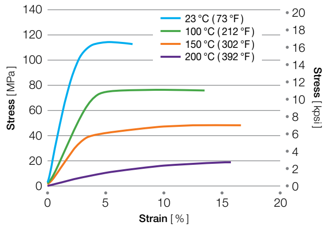
Figure 3.31 Stress-strain curves for AvaSpire® AV-722 BG20
