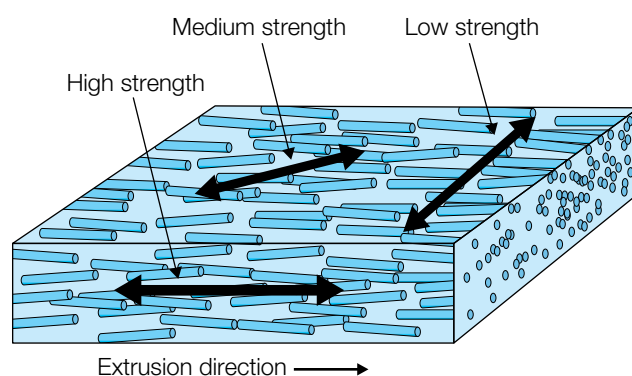
Figure 10.11 Fiber orientation affects strength
