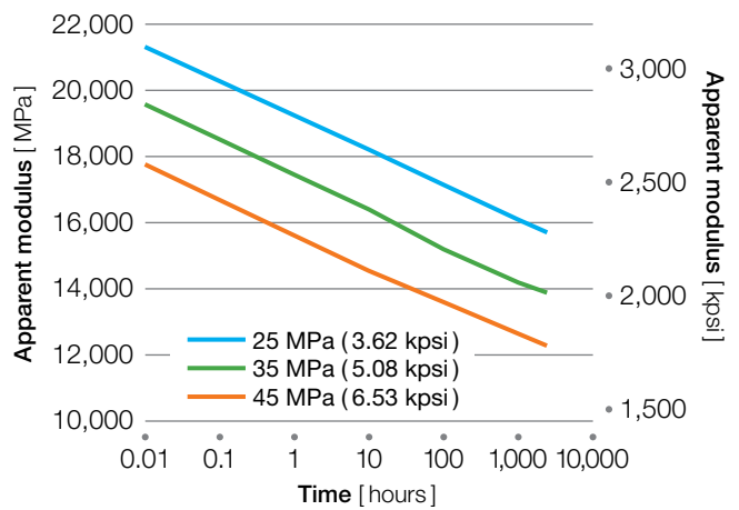
Figure 4.12 AV-722 CF30 at 120 °C (248 °F)
