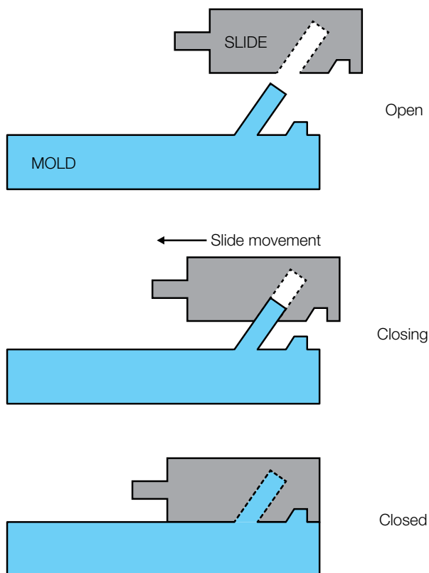
Figure 9.21 Angled pin slide schematic
