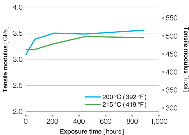
Figure 7.10 Tensile modulus of AV-621 NT after high-temperature aging
