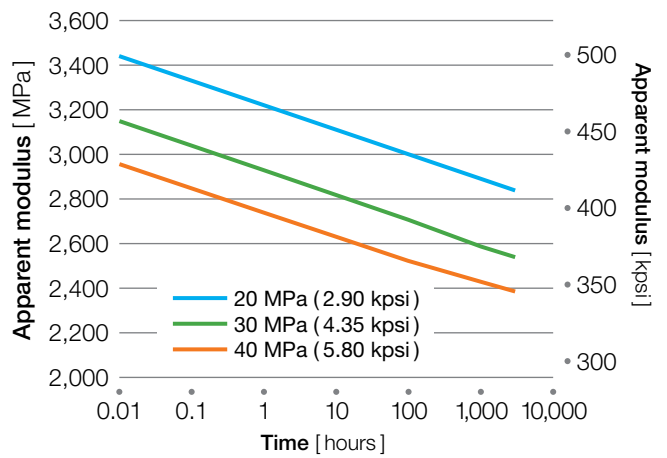
Figure 4.5 AV-621 NT at 23 °C (73 °F)
