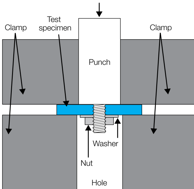
Figure 3.35 Diagram of shear test apparatus
