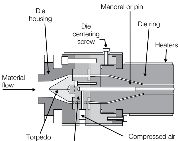
Figure 9.30 Tubing die
