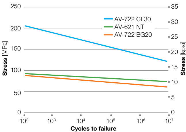
Figure 4.19 Tensile fatigue of AvaSpire® PAEK at 23 °C (73 °F)
