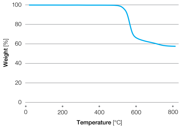
Figure 5.14 TGA AV-621 NT in N2
