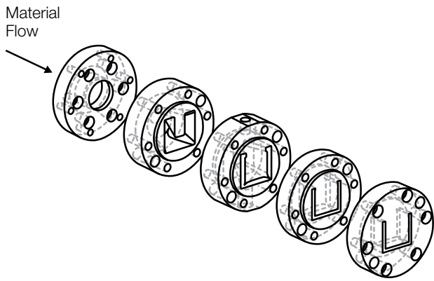
Figure 9.32 Typical profile extrusion die
