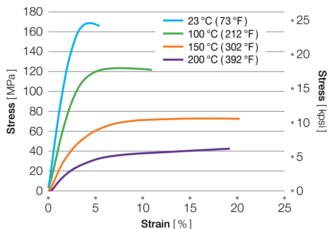
Figure 3.32 Stress-strain curves for AvaSpire® AV-722 CF30
