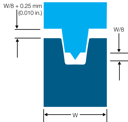
Figure 10.6 Shear joint
