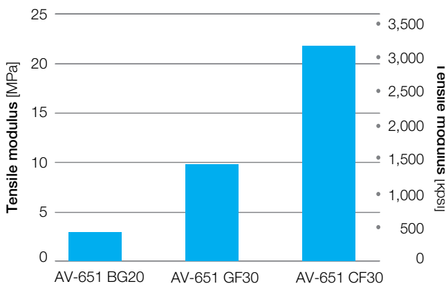
Figure 3.5 Tensile modulus and fiber reinforcement
