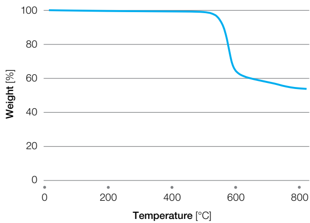
Figure 5.16 TGA AV-651 BG15 in N2
