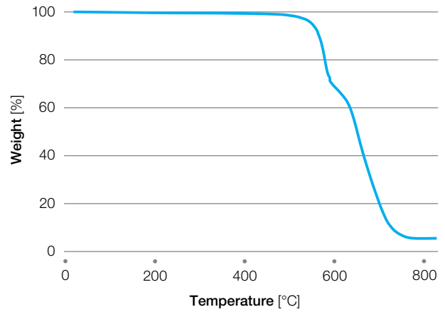
Figure 5.11 TGA AV-651 BG15 in Air
