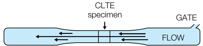
Figure 5.2 CLTE specimen
