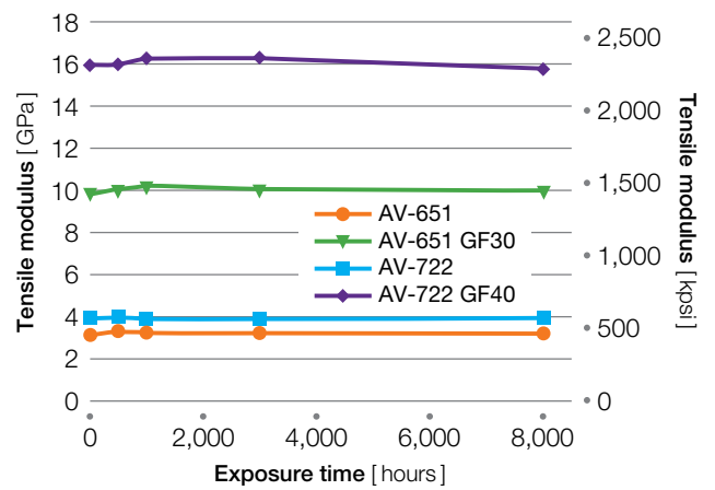
Figure 7.16 Tensile modulus
