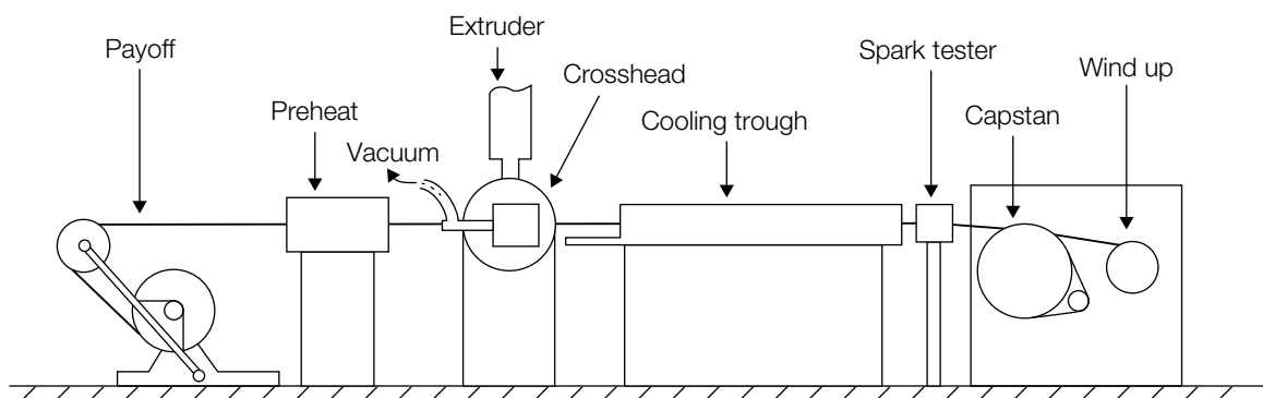
Figure 9.34 Typical wire extrusion equipment
