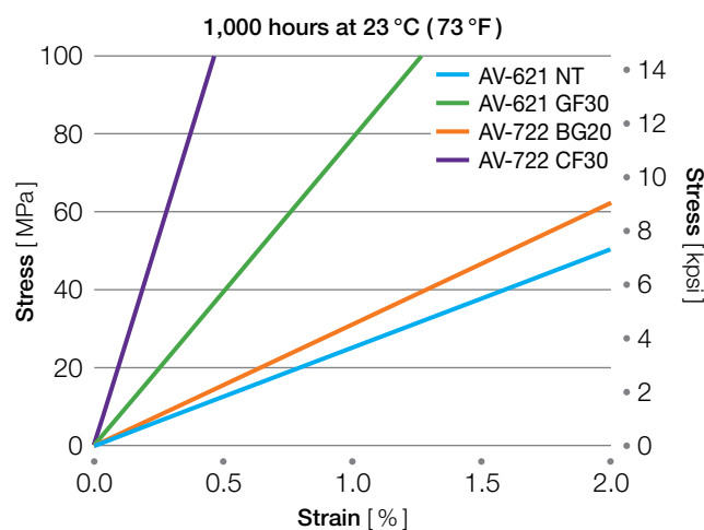
Figure 4.1 Isochronous curves at 23 °C (73 °F)
