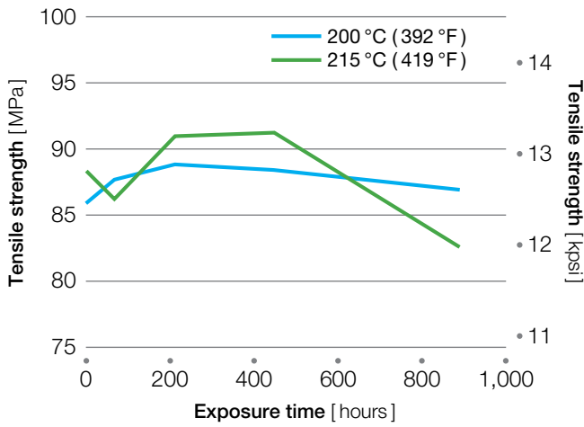
Figure 7.8 Tensile strength of AV-621 NT after high-temperature aging
