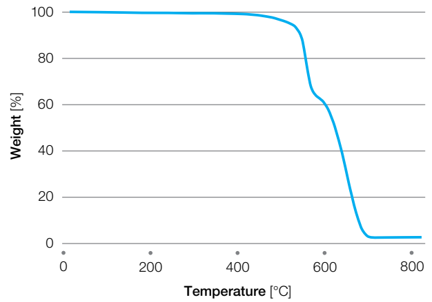
Figure 5.12 TGA AV-722 BG20 in Air
