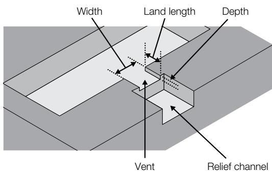
Figure 9.25 Vents
