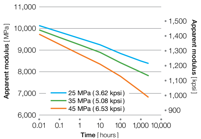
Figure 4.11 AV-621 GF30 at 120 °C (248 °F)
