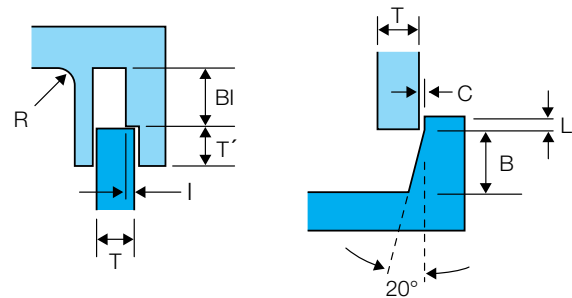
Figure 10.1 Typical spin weld joint designs
