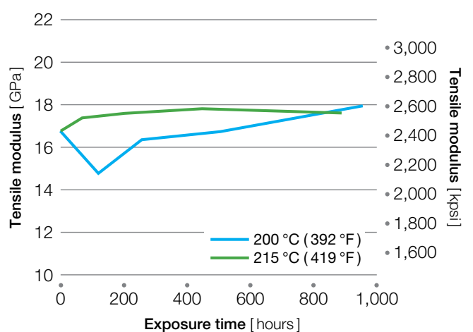
Figure 7.13 Tensile modulus of AV-621 CF30 after high-temperature aging
