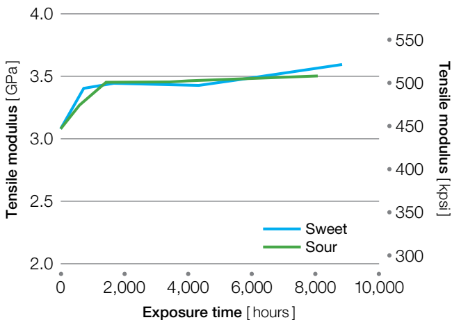
Figure 7.4 Tensile modulus of AV-621 NT exposed at 170 °C (338 °F)
