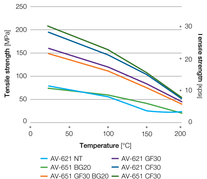
Figure 3.7 Tensile strength vs. temperature AvaSpire® AV-600 Series
