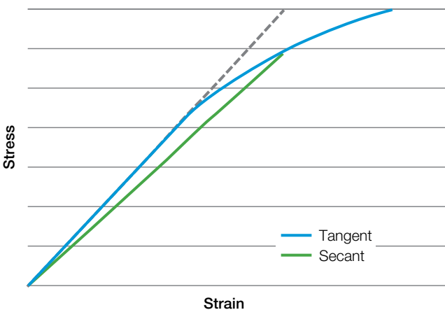
Figure 3.2 Tensile modulus calculation
