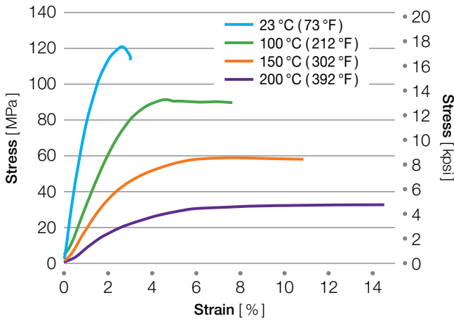
Figure 3.34 Stress-strain curves for AvaSpire® AV-742 SL30
