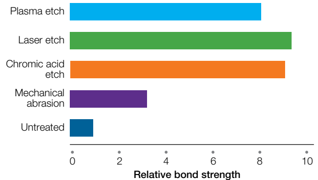
Figure 10.8 Surface preparation and bond strength
