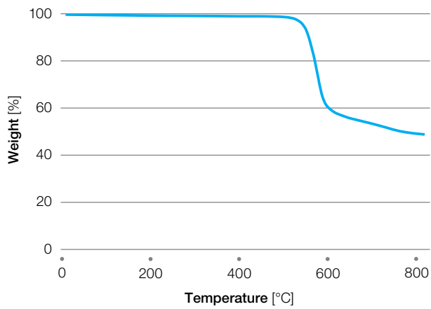
Figure 5.15 TGA AV-630 NT in N2
