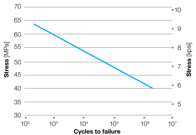
Figure 4.20 Tensile fatigue of AvaSpire® AV-621 GF30 BG20 at 160 °C (320 °F)
