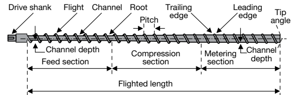
Figure 9.27 Extruder screw schematic
