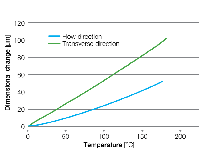
Figure 5.4 CLTE of AvaSpire® AV-621 GF30
