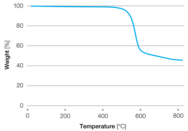
Figure 5.18 TGA AV-848 NT in N2
