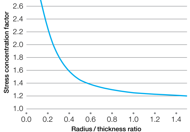
Figure 8.6 Stress concentration at inside corners
