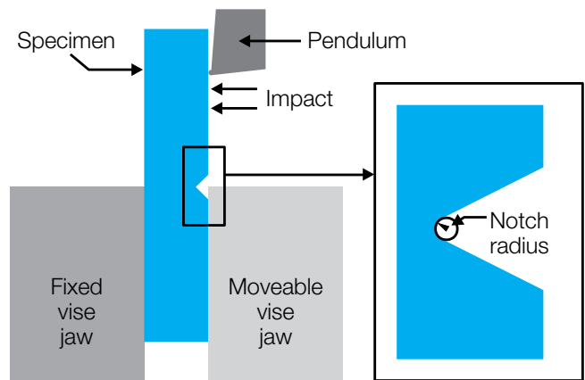
Figure 3.36 Notched Izod specimen
