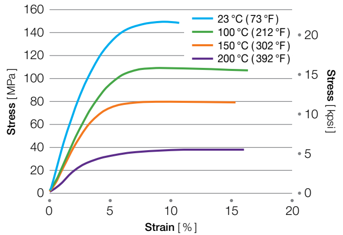
Figure 3.30 Stress-strain curves for AvaSpire® AV-621 CF30
