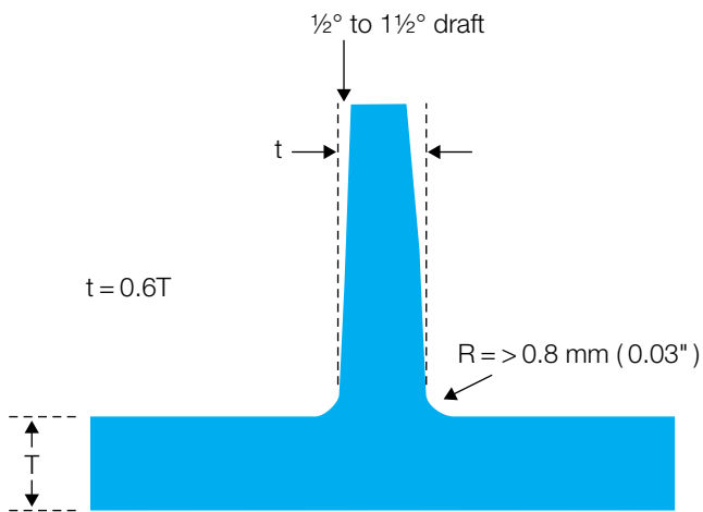
Figure 8.17 Draft – recommended rib design
