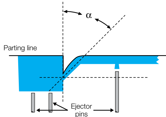
Figure 9.24 Tunnel gate
