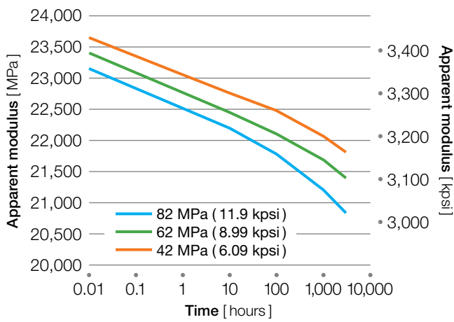
Figure 4.8 AV-722 CF30 at 23 °C (73 °F)
