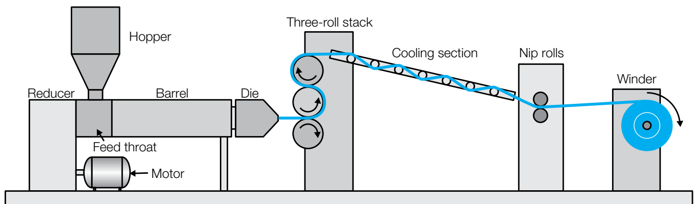
Figure 9.31 Typical three-roll stack
