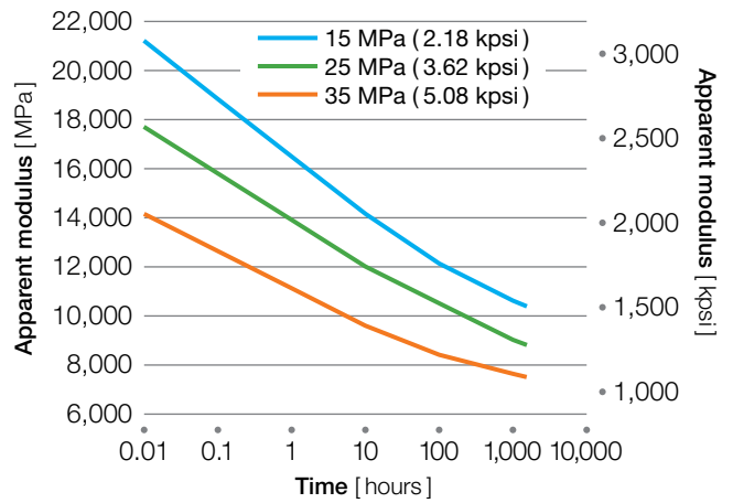
Figure 4.16 AV-848 CF30 at 160 °C (320 °F)
