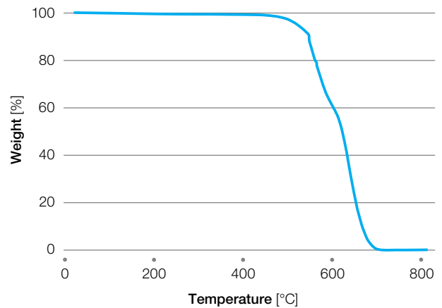
Figure 5.13 TGA AV-848 NT in Air
