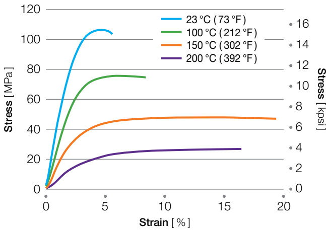
Figure 3.33 Stress-strain curves for AvaSpire® AV-722 SL30
