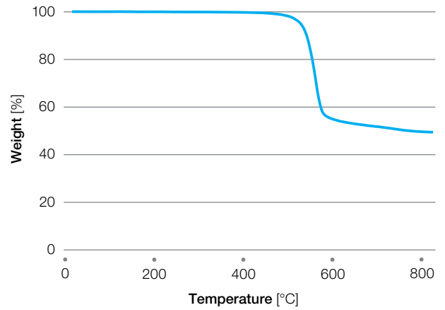
Figure 5.17 TGA AV-722 BG20 in N2
