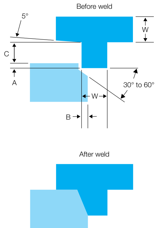
Figure 4: Shear joint
