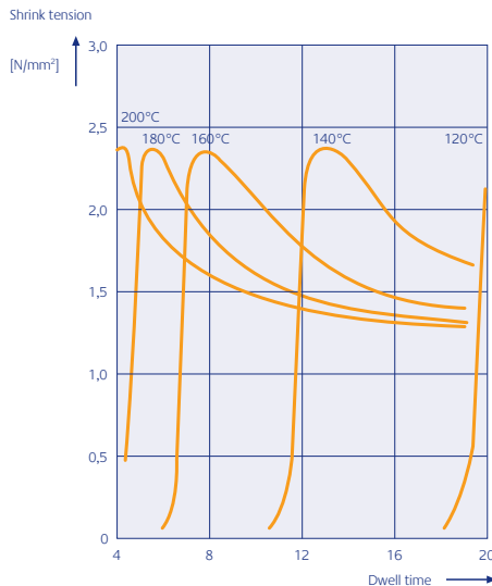
Fig. 23 Effect of dwell time on thermal shrink tension of SABIC® LDPE (MFR 2, density 921). Film thickness 100 microns; BUR 1.5; Temperatures 120°C, 140°C, 160°C, 180°C and 200°C.
