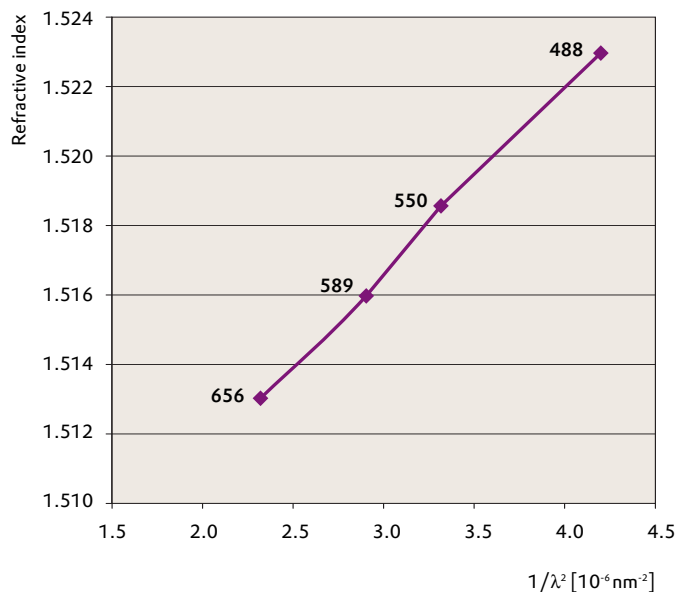
Figure 2: Refractive index of TROGAMID CX7323 (T = 20 °C)
