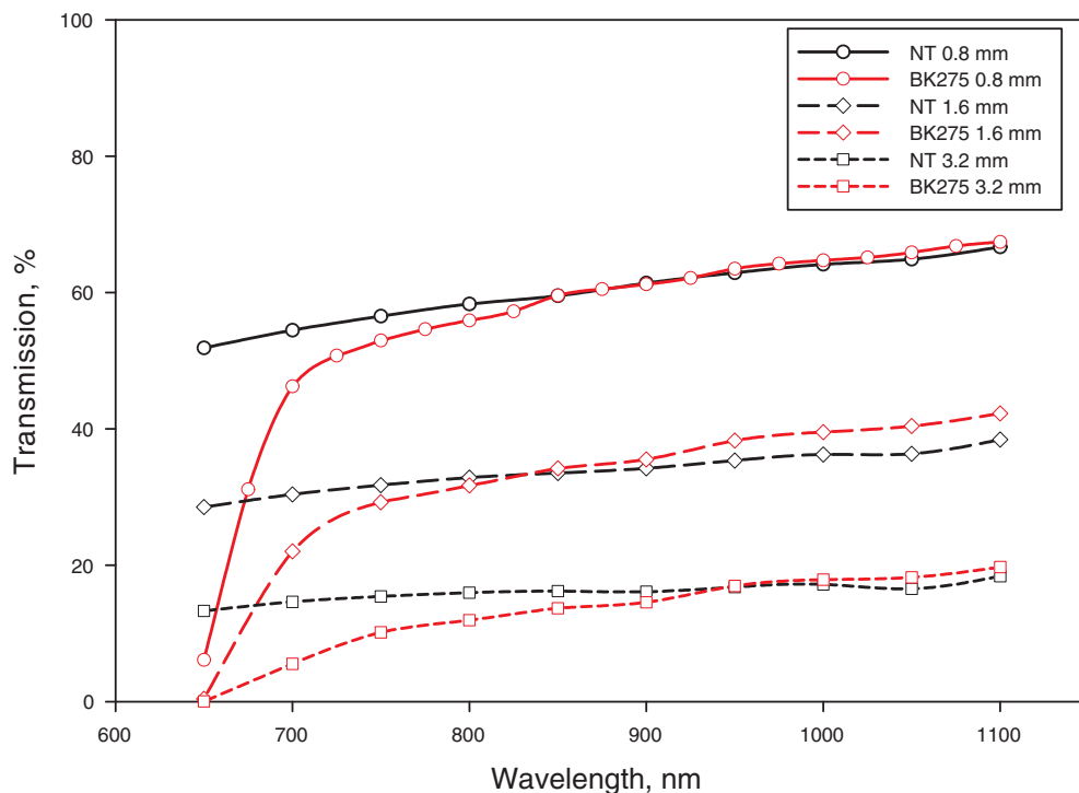
Transmissivity of Amodel A-6135 BK275
